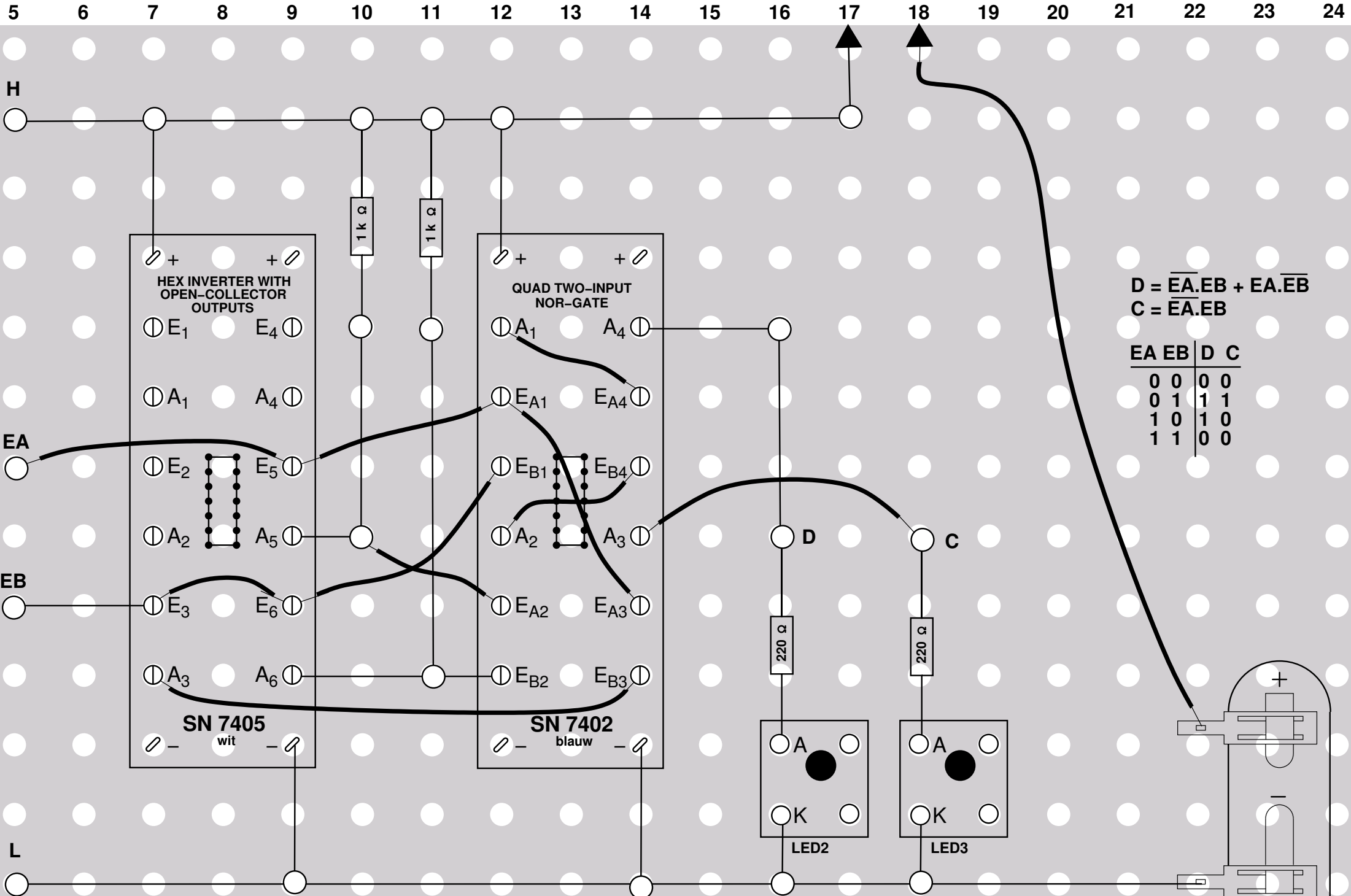
4.10.21. 1-bit subtract
